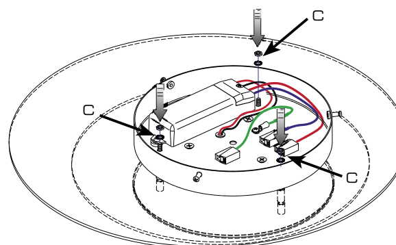
Atornillar C Screw C
