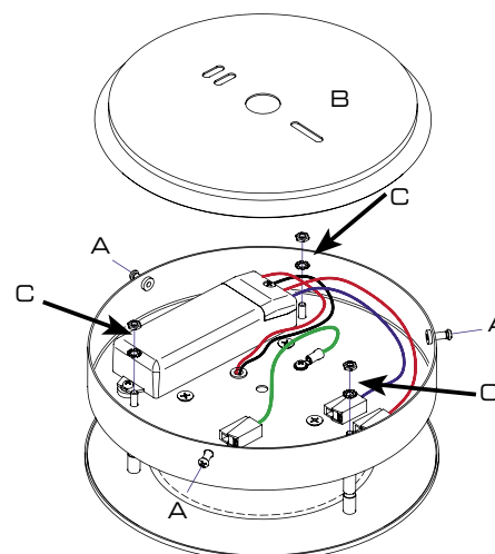
Desenroscar A y C Unscrew A and C
