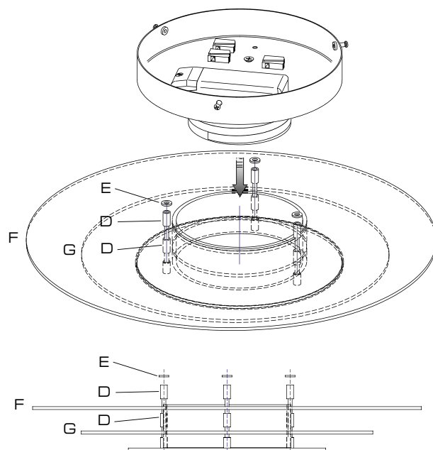
Insertar pantallas G y F entre separadores D y E Insert shades G and F between separators D and E
